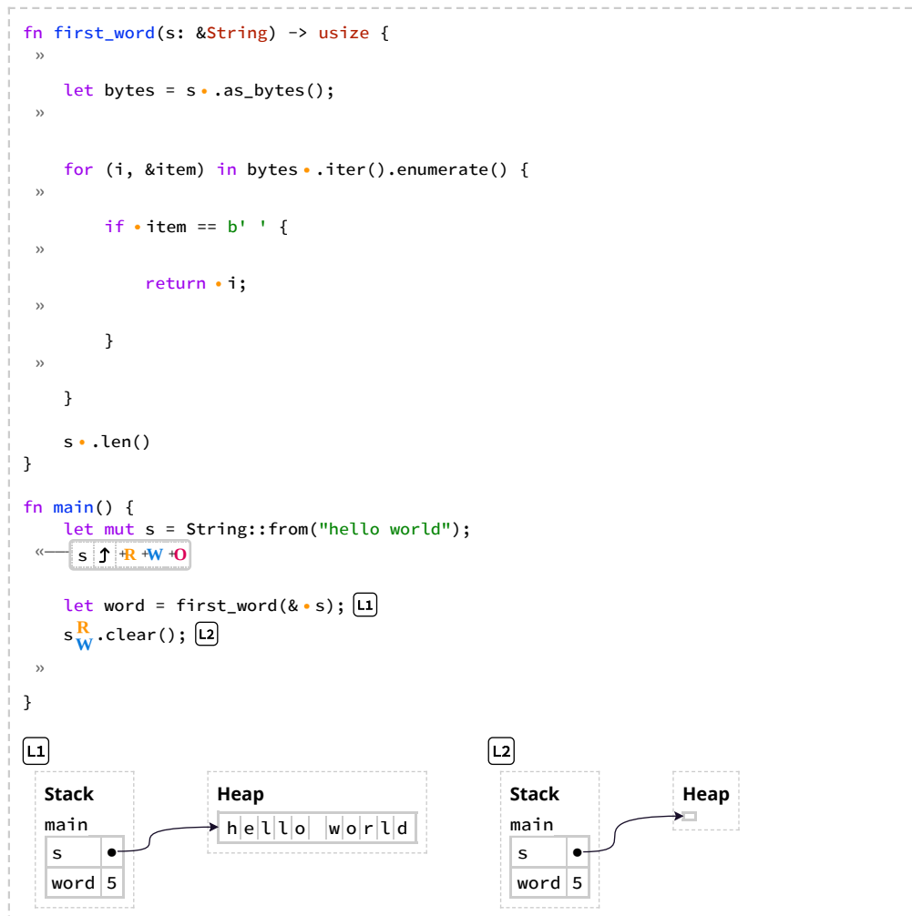
Listing 4-8: Storing the result from calling the first_word function and then changing the String contents
