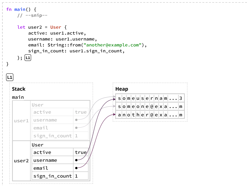
Listing 5-6: Creating a new User instance using all but one of the values from user1
